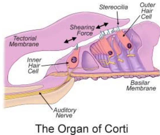
Figure 1.1.3 – The Organ of Corti, showing the membrane arrangement and the inner and outer hair cells.
